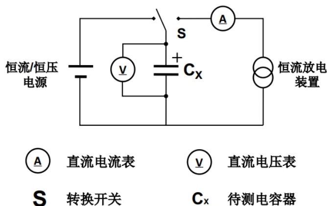
Figure 1 Constant current discharge circuit for measuring 图1 恒流放电方法电路
