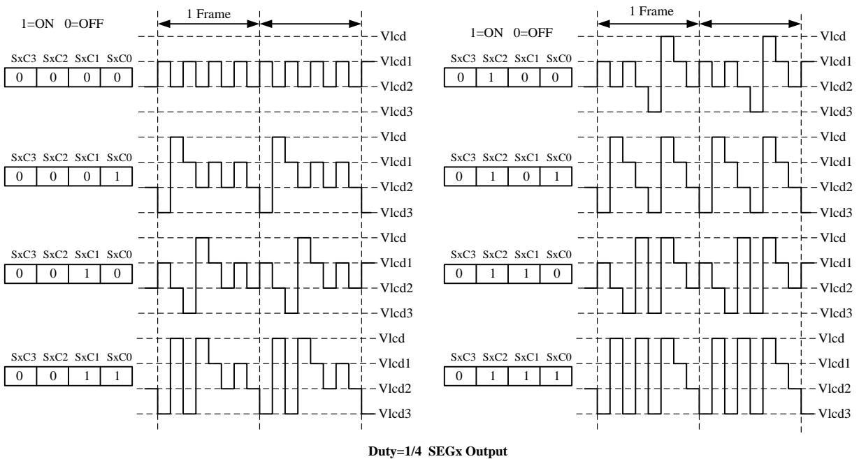
SEGMENT 输出波形(1/4 Duty):
